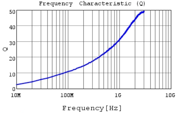
LQP03TN2N7B02 Q
