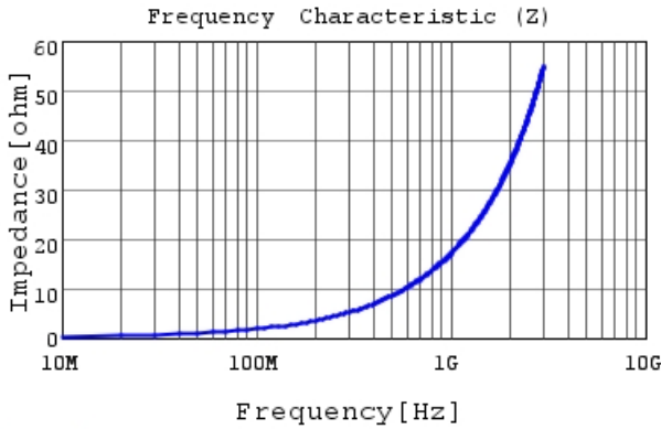
LQP03TN2N7B02 |Z|
