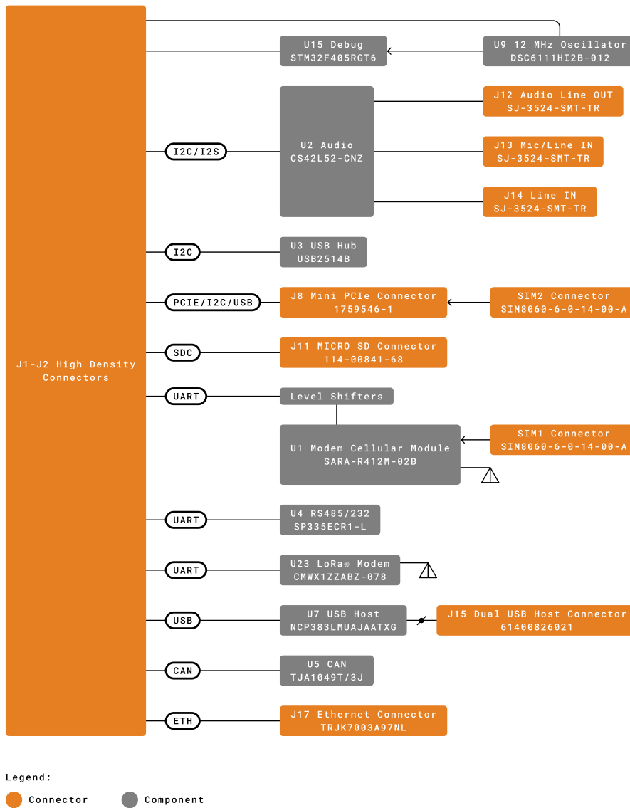
Block Diagram
